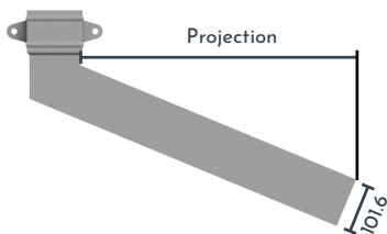
Eared Long Tail Elbow 112.5° & 135° - Left & Right Handed
