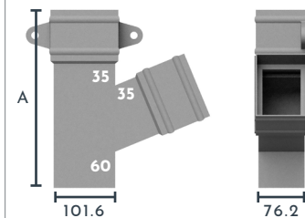
Eared Left/Right Hand Branches
