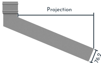
Non-Eared Long Tail Elbow 112.5° & 135°
