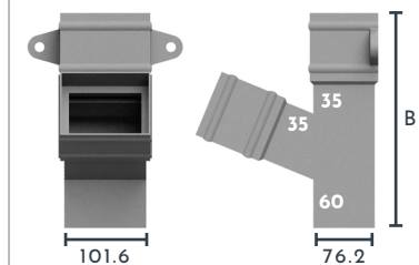
Eared Front Hand Branch
